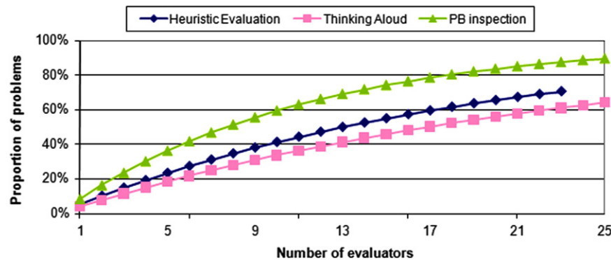
Fig. 4. The cost-benefit curve for the three evaluation techniques.
